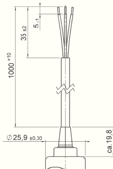
Flying leads
